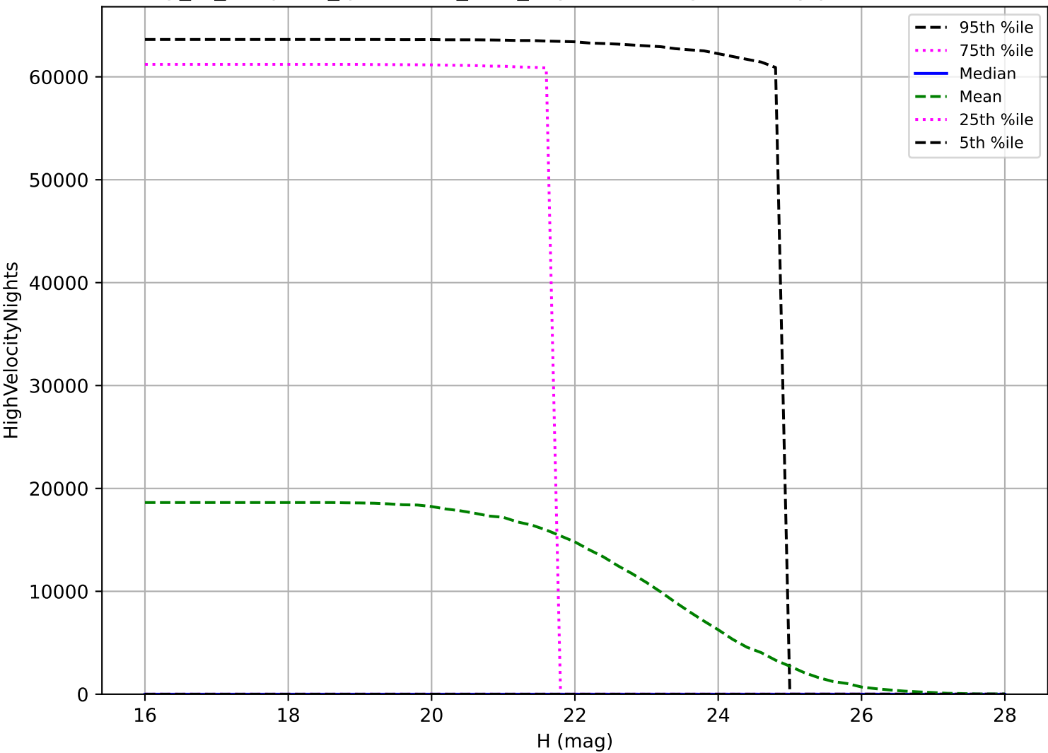
early_ss_template_fpextra2.0_v3.4_10yrs: NEO High velocity pair detection loss
