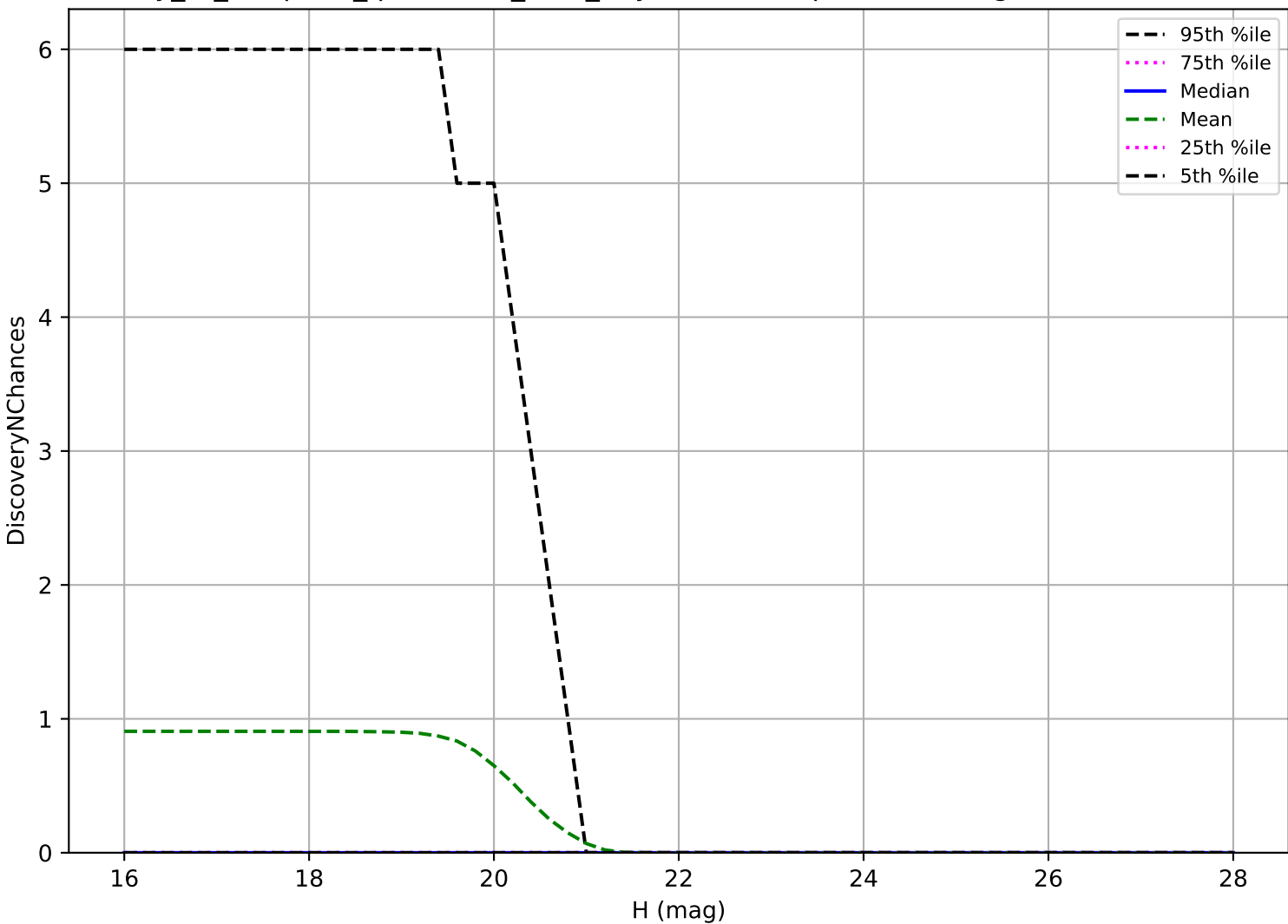
early_ss_template_fpextra2.0_v3.4_10yrs: Vatira 3 pairs in 15 nights detection loss
