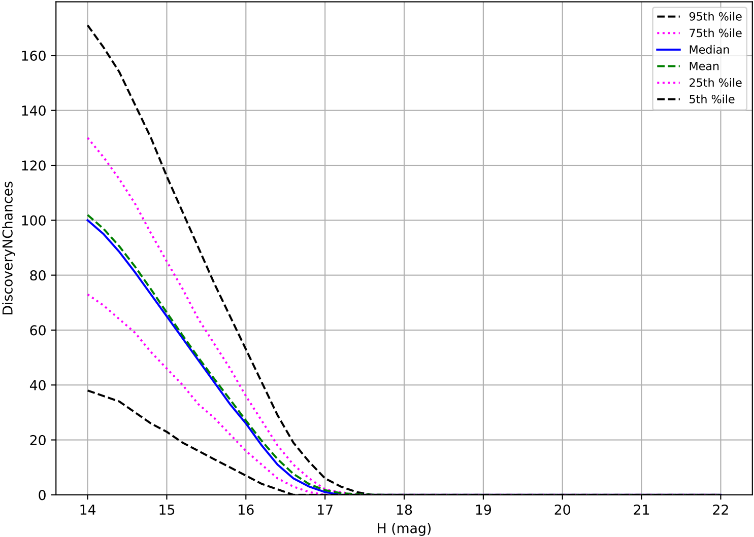
early_ss_template_fpextra2.0_v3.4_10yrs: Trojan 3 pairs in 15 nights detection loss
