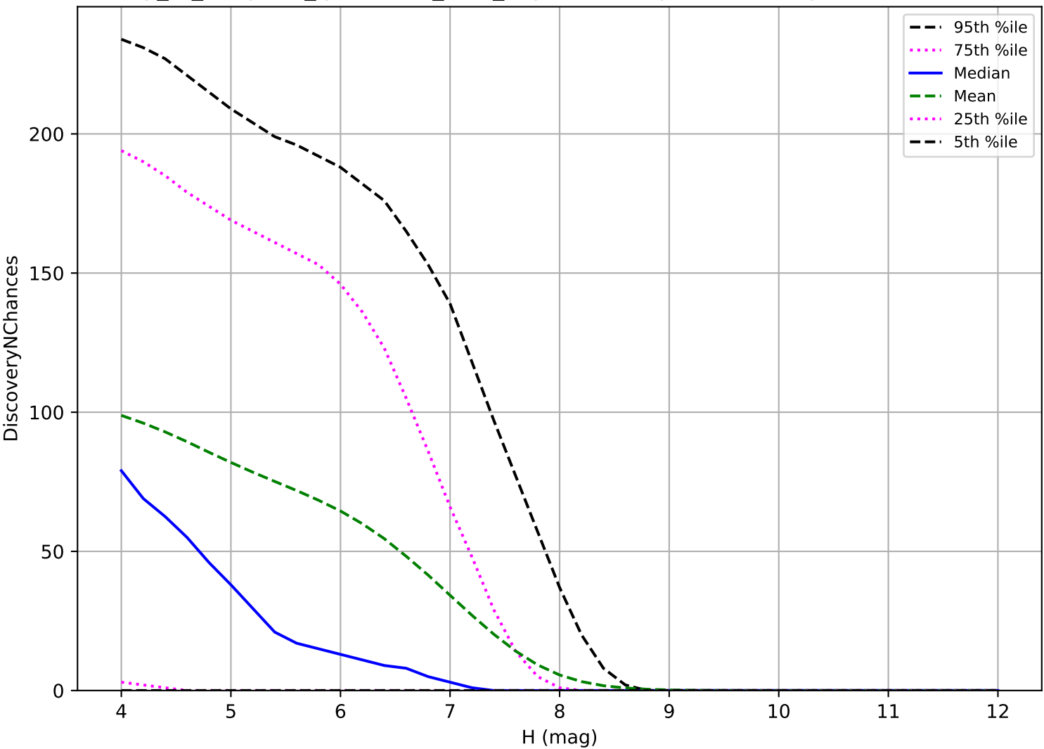
early_ss_template_fpextra2.0_v3.4_10yrs: TNO 3 pairs in 15 nights detection loss
