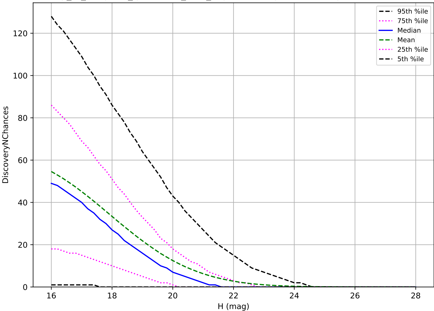
early_ss_template_fpextra2.0_v3.4_10yrs: PHA 3 pairs in 15 nights detection loss
