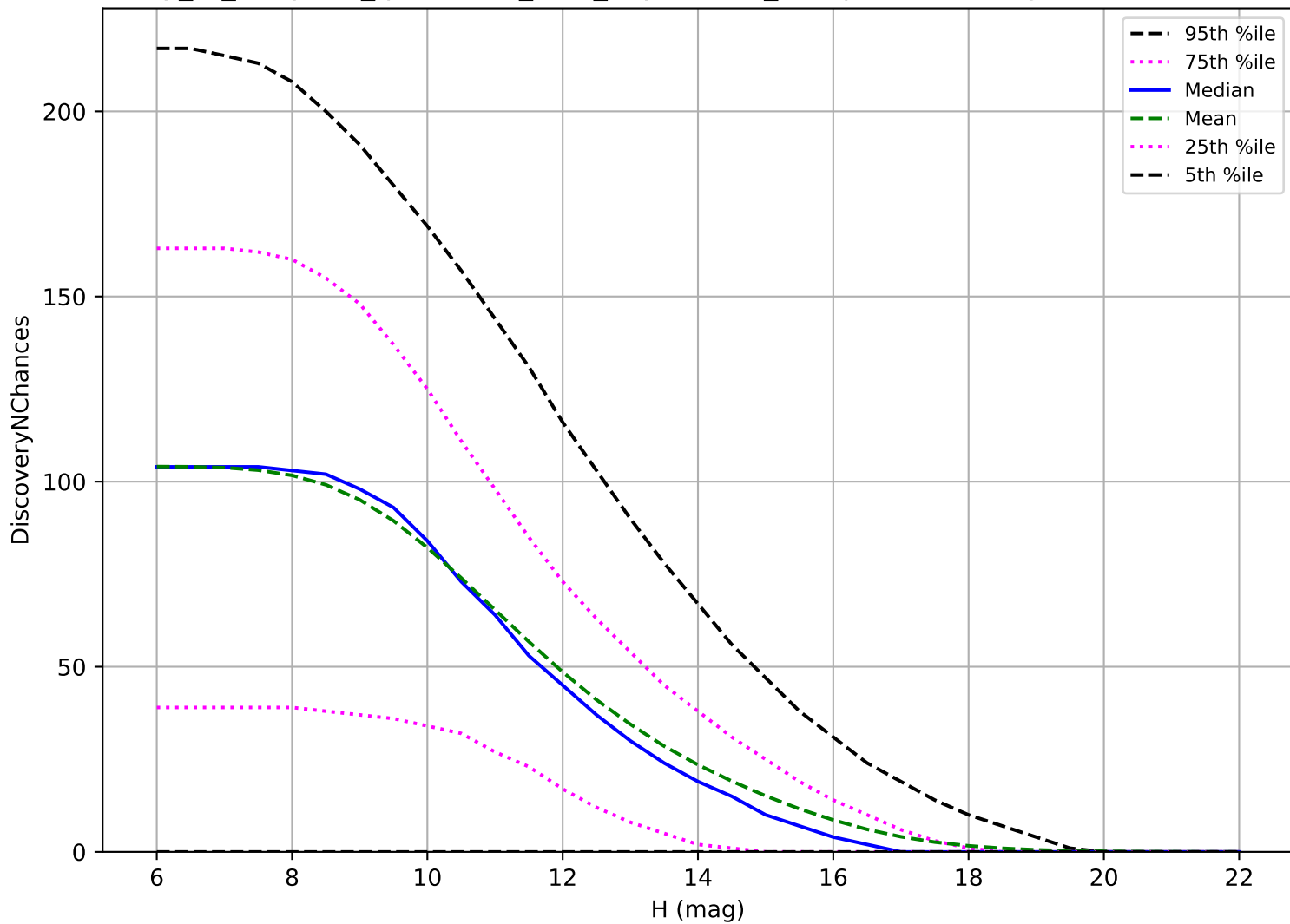
early_ss_template_fpextra2.0_v3.4_10yrs: OCC_r5 3 pairs in 15 nights detection loss
