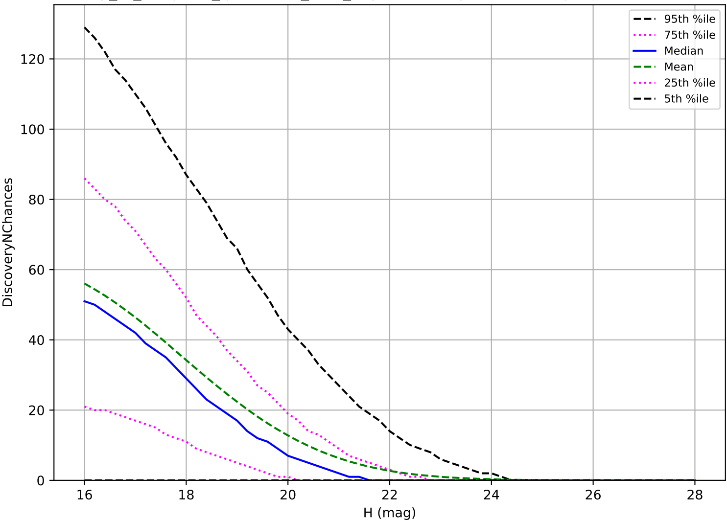
early_ss_template_fpextra2.0_v3.4_10yrs: NEO 3 pairs in 15 nights detection loss
