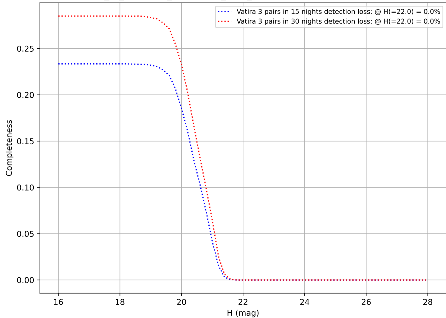
early_ss_template_fpextra2.0_v3.4_10yrs: DifferentialCompleteness
