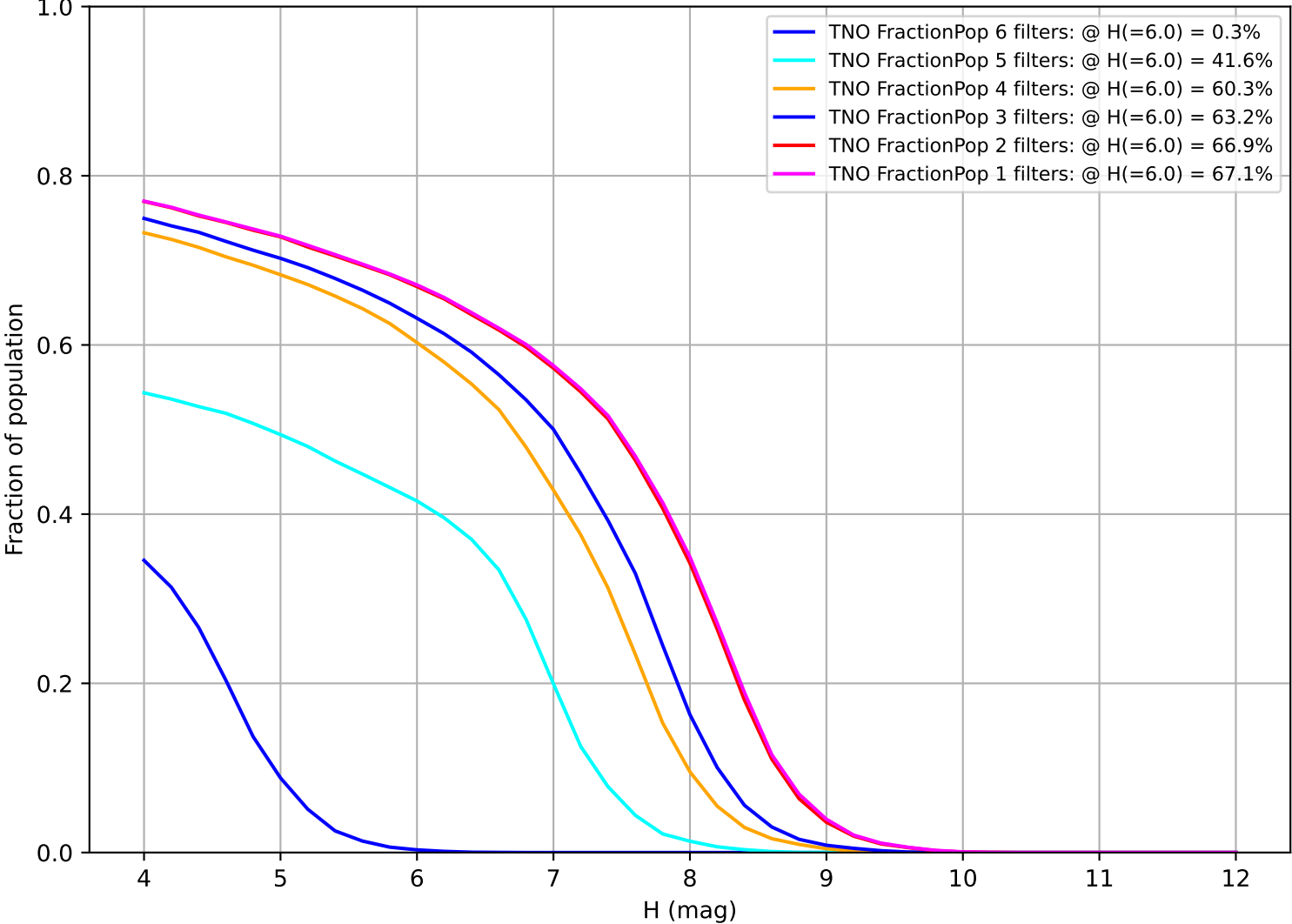
early_ss_template_fpextra2.0_v3.4_10yrs: Fraction of population with colors in X filters TNO
