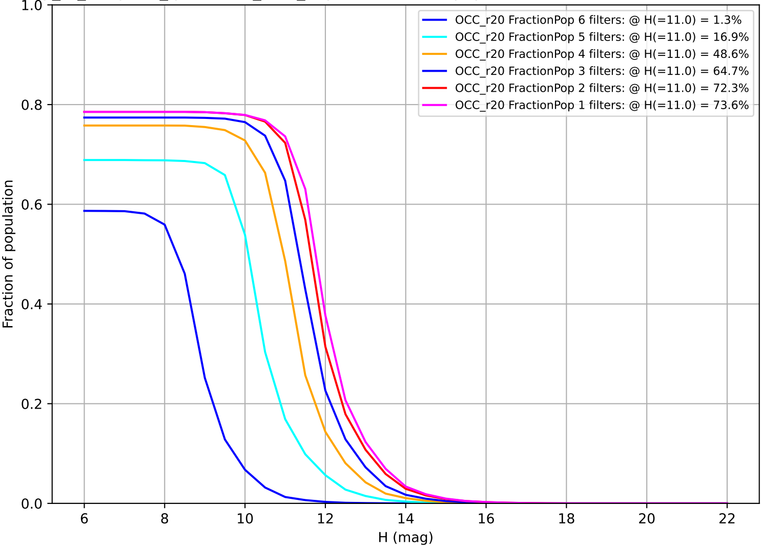
early_ss_template_fpextra2.0_v3.4_10yrs: Fraction of population with colors in X filters OCC_r20
