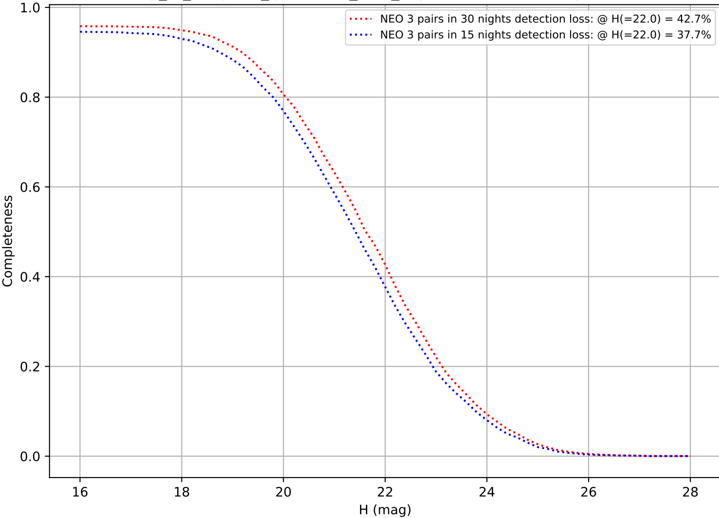
early_ss_template_fpextra2.0_v3.4_10yrs: DifferentialCompleteness
