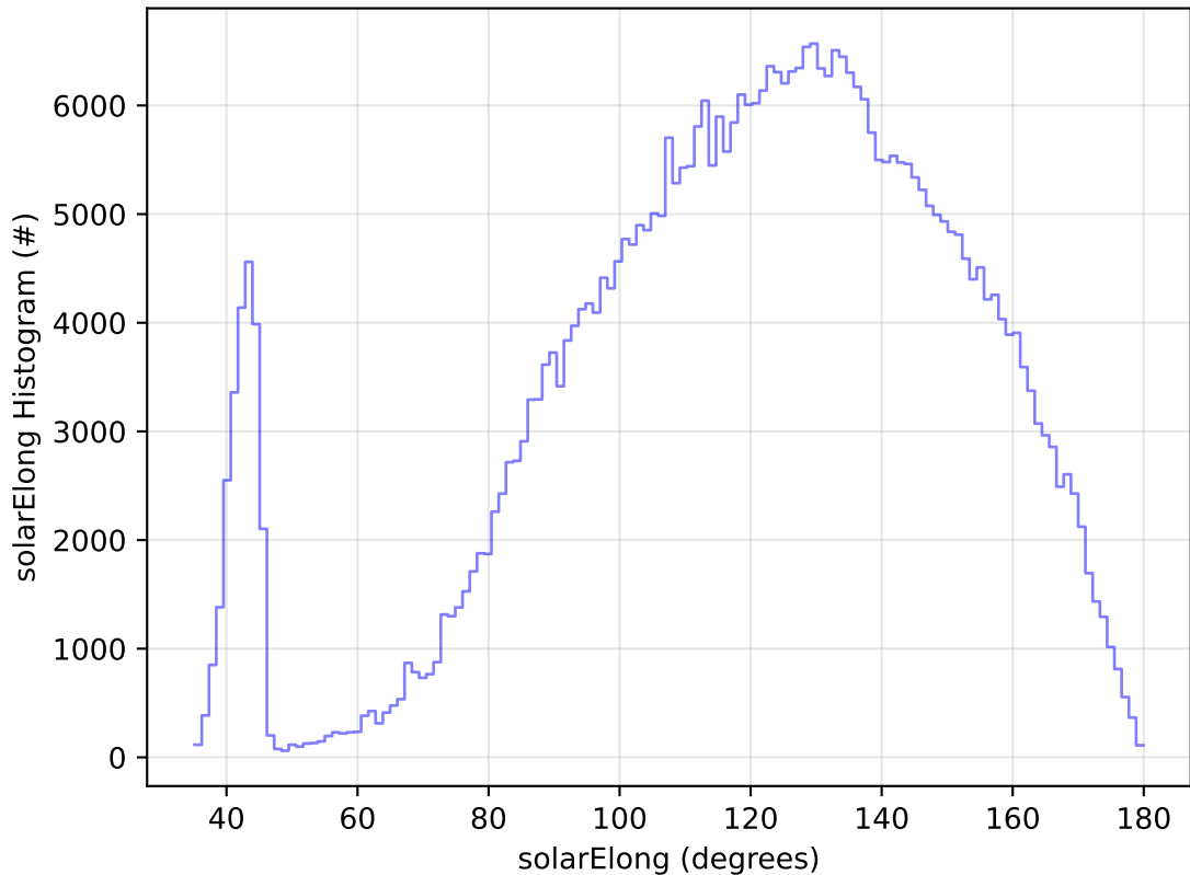
early_ss_template_fpextra2.0_v3.4_10yrs WFD z band: solarElong Histogram
