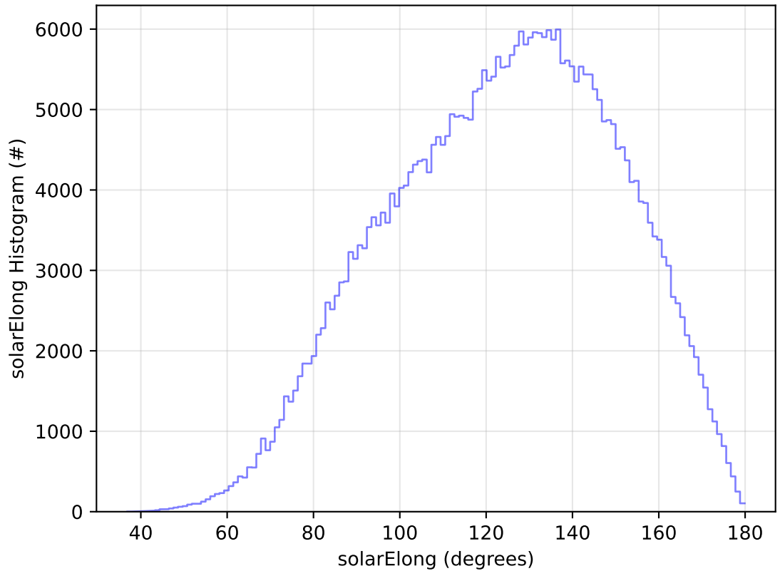
early_ss_template_fpextra2.0_v3.4_10yrs WFD y band: solarElong Histogram
