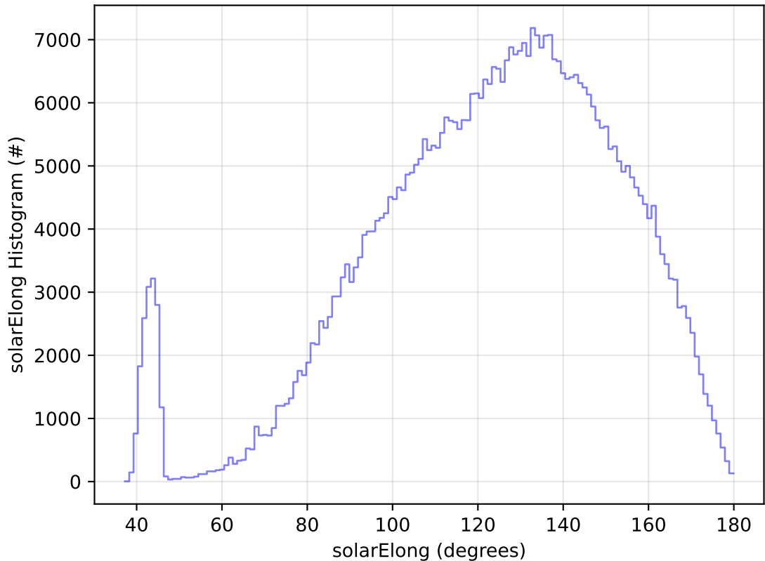
early_ss_template_fpextra2.0_v3.4_10yrs WFD r band: solarElong Histogram
