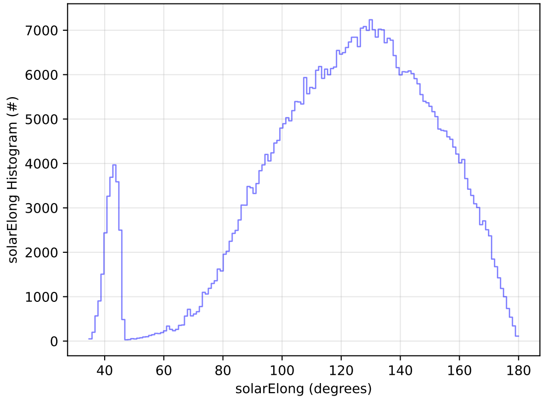
early_ss_template_fpextra2.0_v3.4_10yrs WFD i band: solarElong Histogram
