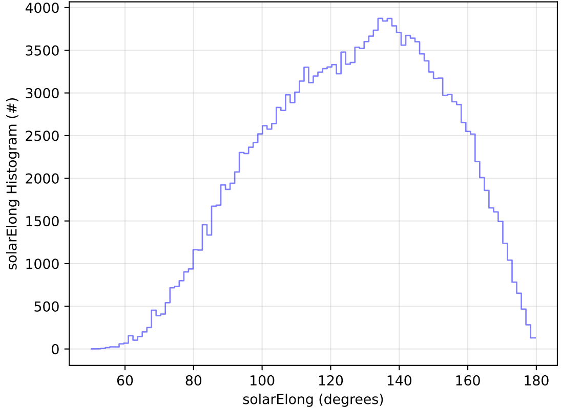
early_ss_template_fpextra2.0_v3.4_10yrs WFD g band: solarElong Histogram
