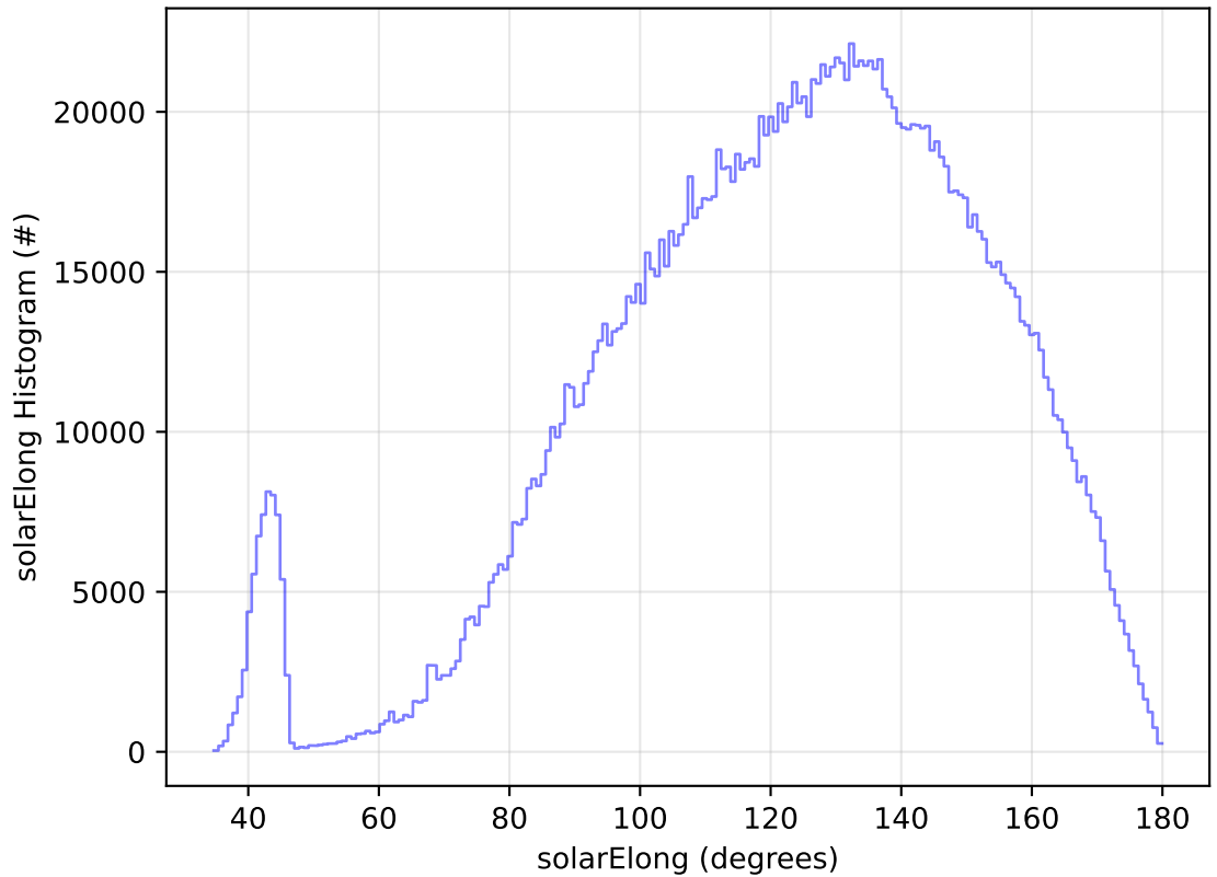
early_ss_template_fpextra2.0_v3.4_10yrs WFD all bands: solarElong Histogram
