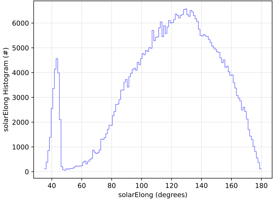
early_ss_template_fpextra2.0_v3.4_10yrs All sky z band: solarElong Histogram
