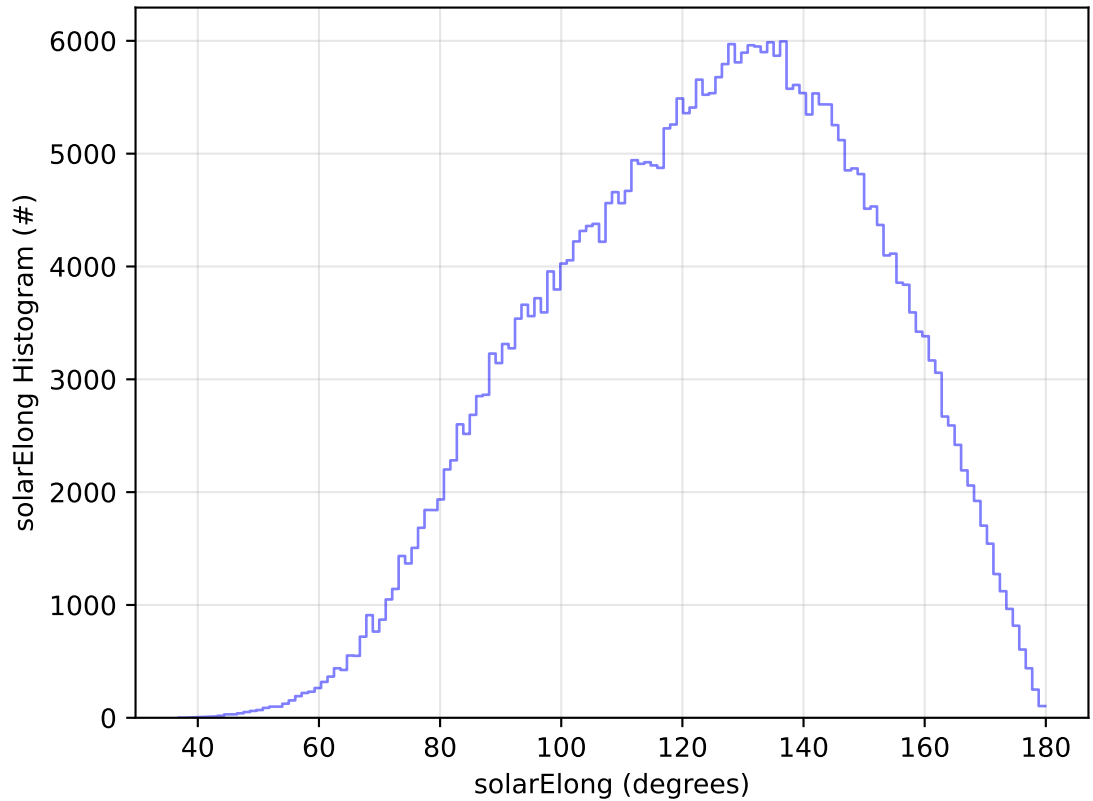
early_ss_template_fpextra2.0_v3.4_10yrs All sky y band: solarElong Histogram
