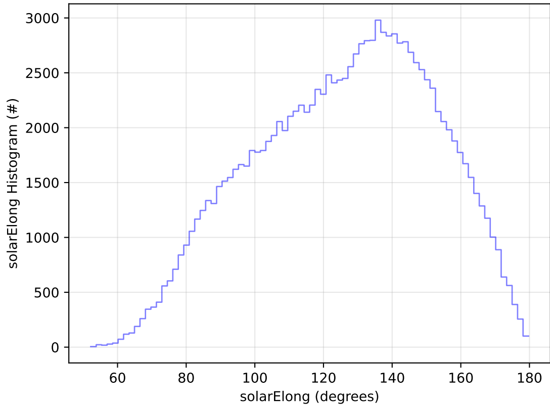
early_ss_template_fpextra2.0_v3.4_10yrs All sky u band: solarElong Histogram
