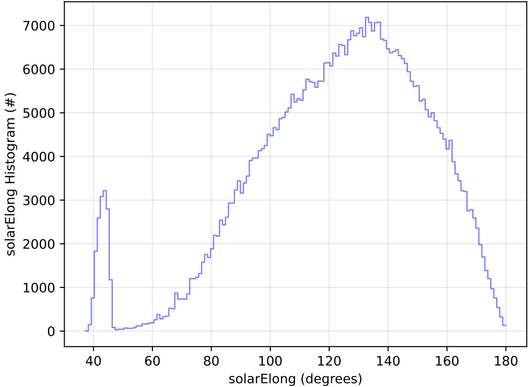
early_ss_template_fpextra2.0_v3.4_10yrs All sky r band: solarElong Histogram
