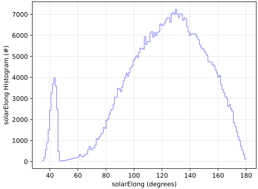
early_ss_template_fpextra2.0_v3.4_10yrs All sky i band: solarElong Histogram
