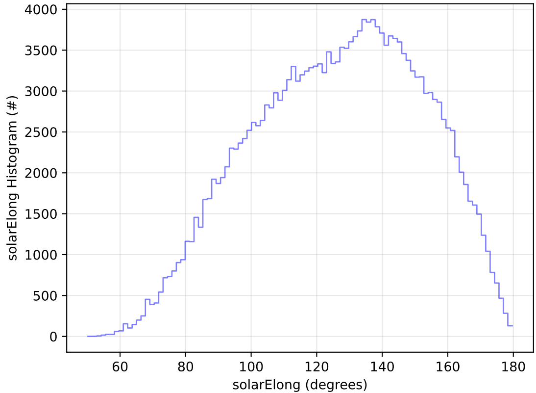
early_ss_template_fpextra2.0_v3.4_10yrs All sky g band: solarElong Histogram
