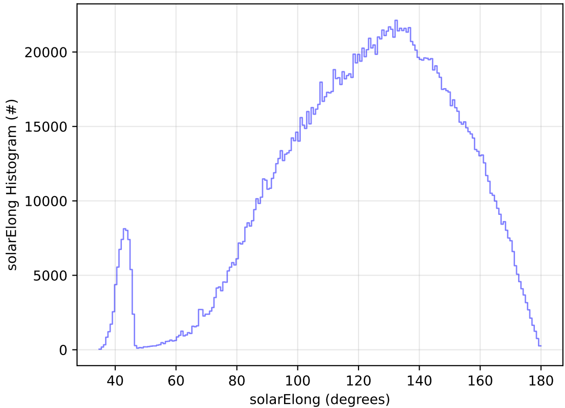
early_ss_template_fpextra2.0_v3.4_10yrs All sky all bands: solarElong Histogram
