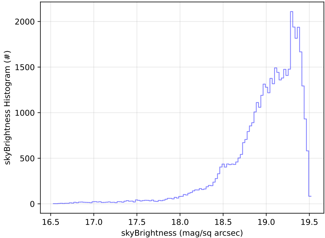
early_ss_template_fpextra2.0_v3.4_10yrs Yr 1 z band: skyBrightness Histogram
