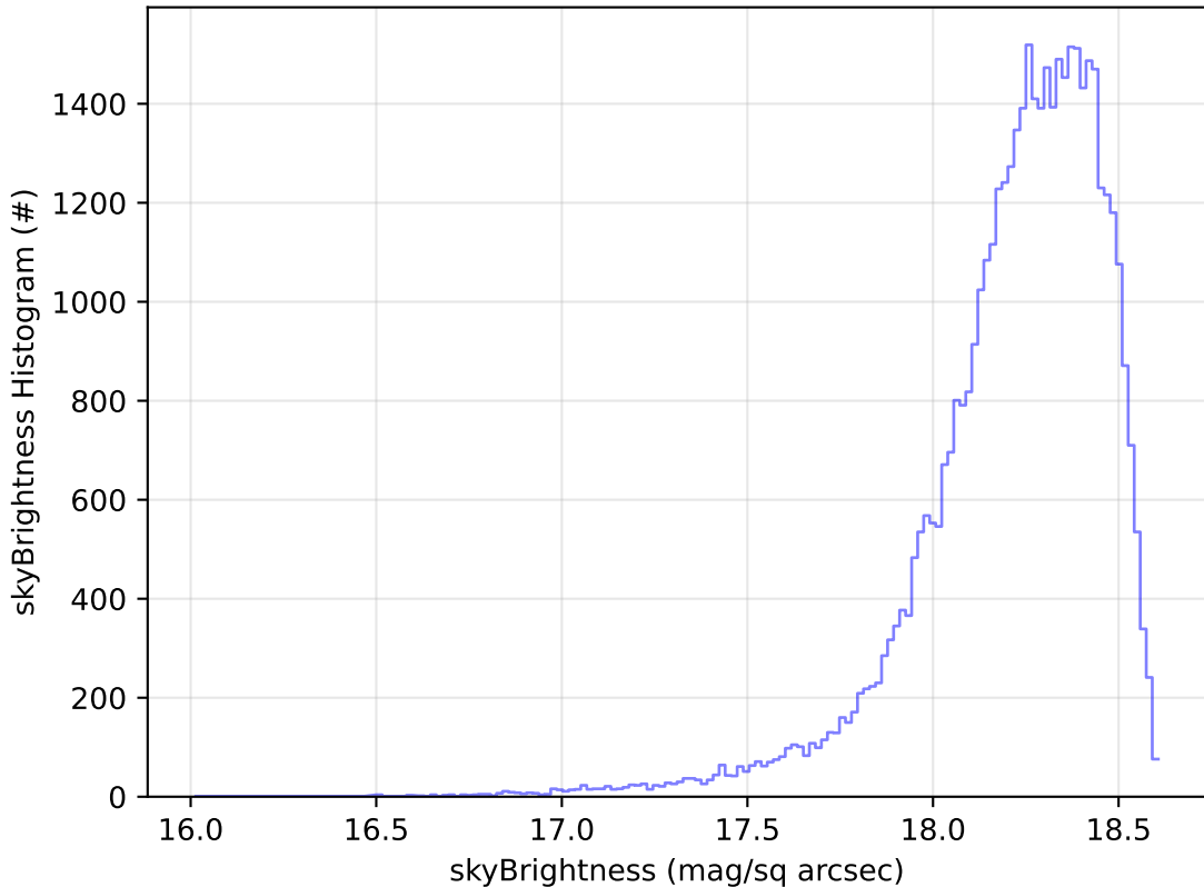
early_ss_template_fpextra2.0_v3.4_10yrs Yr 1 y band: skyBrightness Histogram
