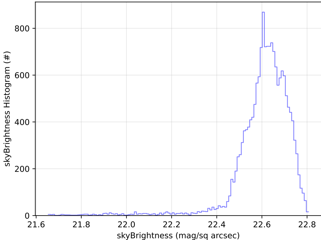
early_ss_template_fpextra2.0_v3.4_10yrs Yr 1 u band: skyBrightness Histogram
