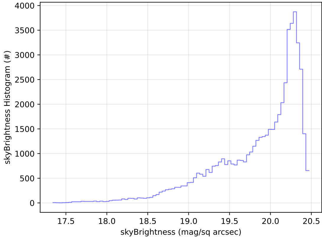
early_ss_template_fpextra2.0_v3.4_10yrs Yr 1 i band: skyBrightness Histogram
