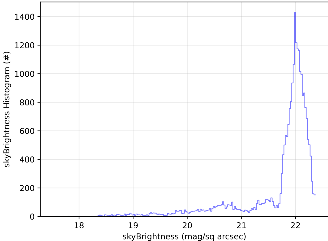
early_ss_template_fpextra2.0_v3.4_10yrs Yr 1 g band: skyBrightness Histogram
