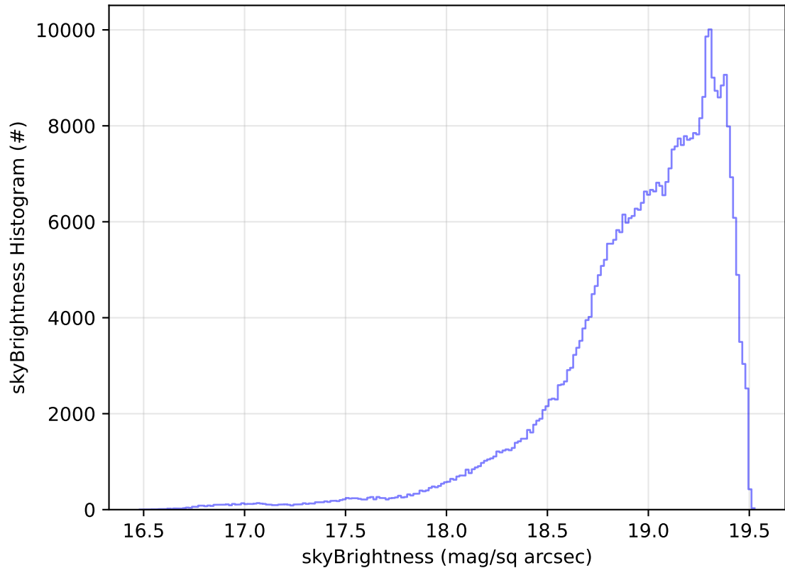
early_ss_template_fpextra2.0_v3.4_10yrs WFD z band: skyBrightness Histogram
