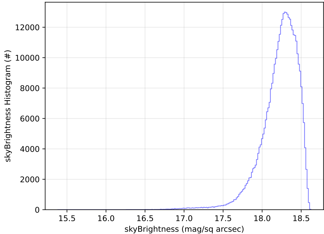
early_ss_template_fpextra2.0_v3.4_10yrs WFD y band: skyBrightness Histogram
