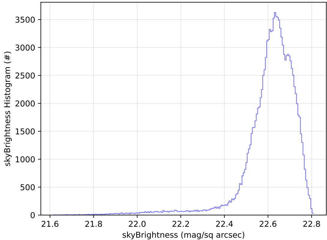
early_ss_template_fpextra2.0_v3.4_10yrs WFD u band: skyBrightness Histogram
