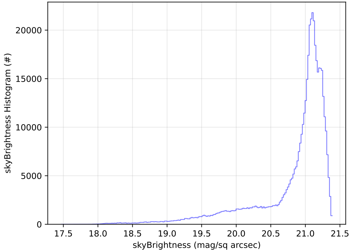
early_ss_template_fpextra2.0_v3.4_10yrs WFD r band: skyBrightness Histogram
