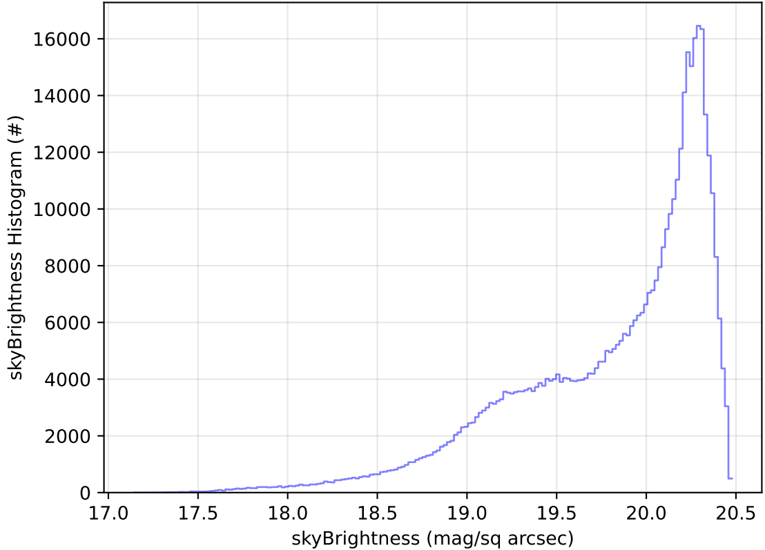
early_ss_template_fpextra2.0_v3.4_10yrs WFD i band: skyBrightness Histogram
