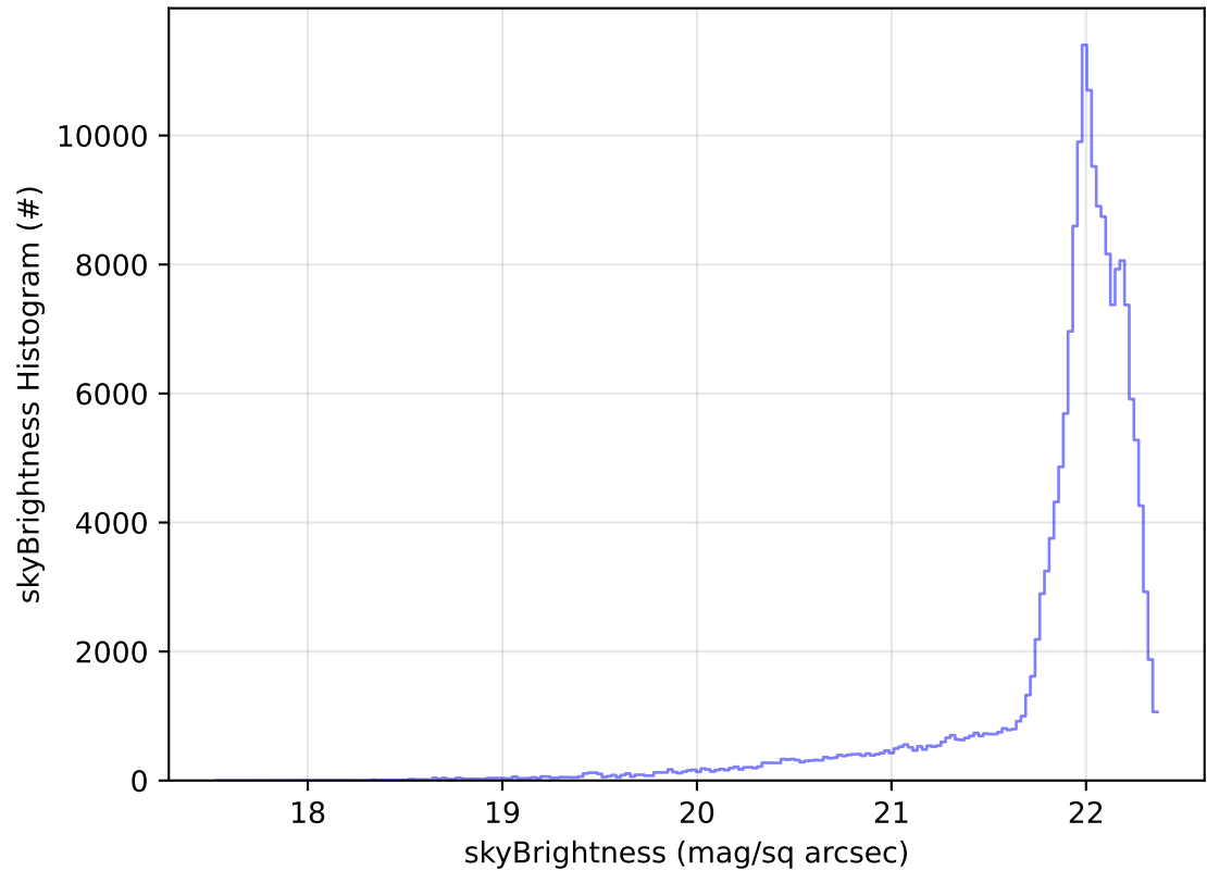
early_ss_template_fpextra2.0_v3.4_10yrs WFD g band: skyBrightness Histogram
