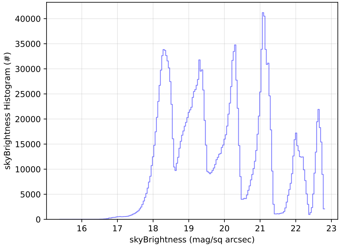
early_ss_template_fpextra2.0_v3.4_10yrs WFD all bands: skyBrightness Histogram
