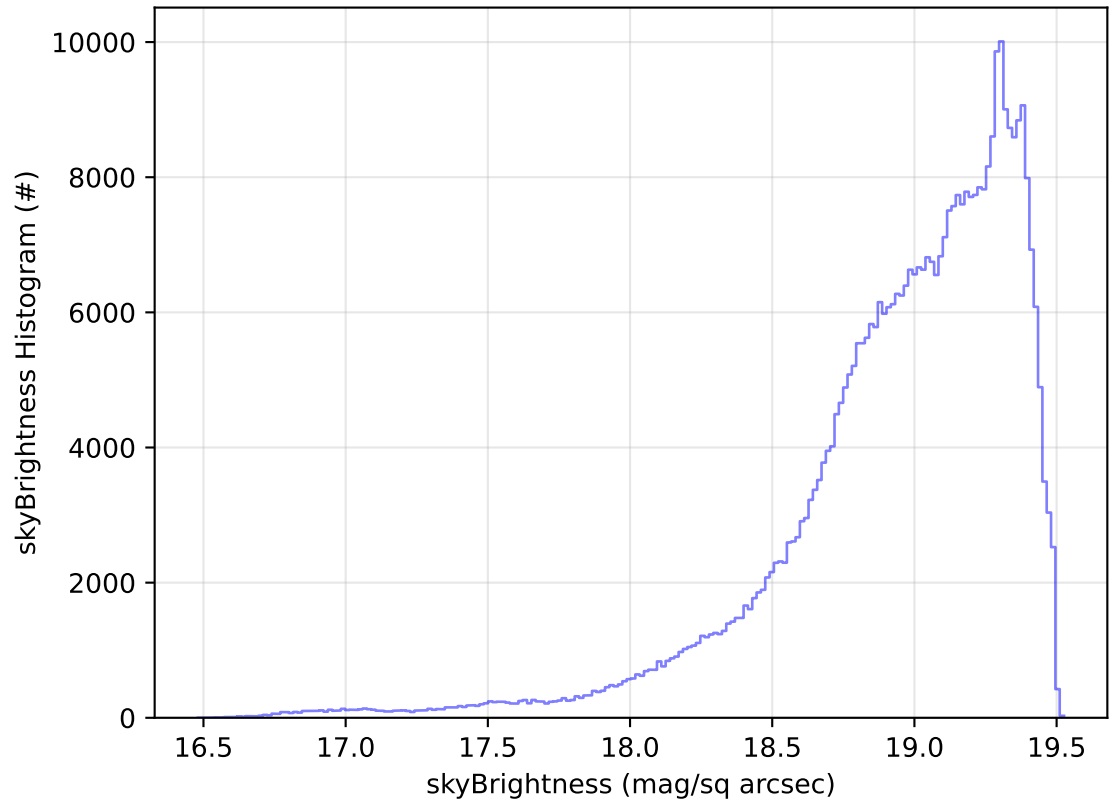
early_ss_template_fpextra2.0_v3.4_10yrs All sky z band: skyBrightness Histogram
