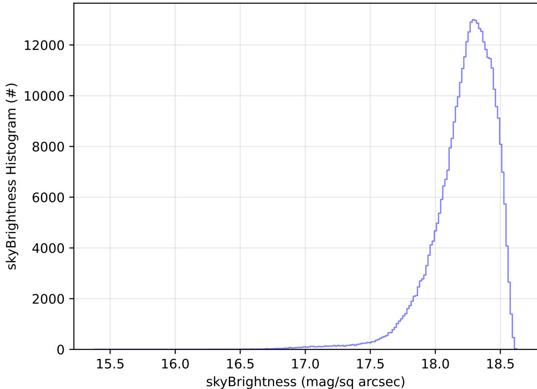
early_ss_template_fpextra2.0_v3.4_10yrs All sky y band: skyBrightness Histogram
