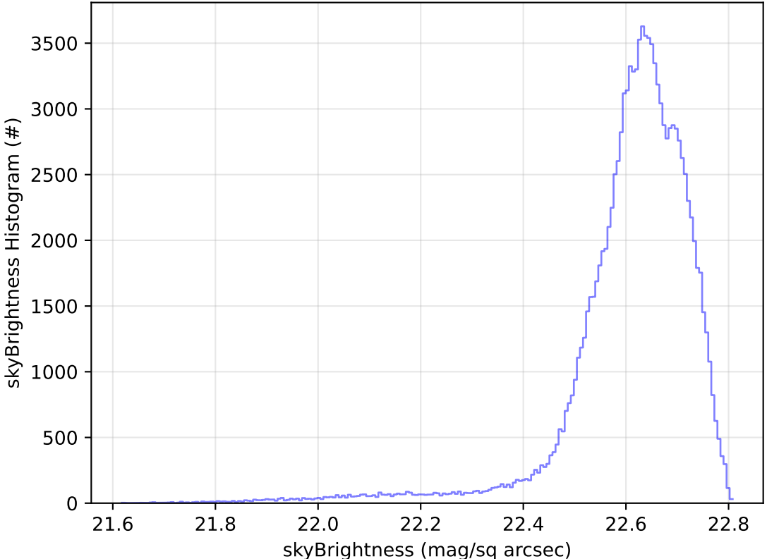
early_ss_template_fpextra2.0_v3.4_10yrs All sky u band: skyBrightness Histogram
