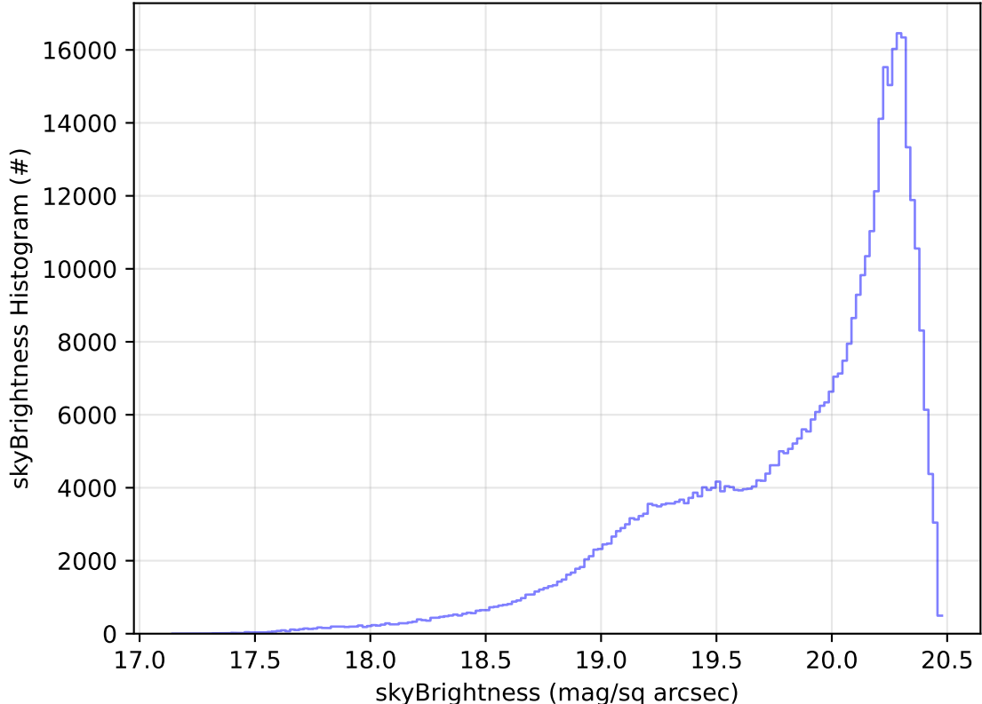
early_ss_template_fpextra2.0_v3.4_10yrs All sky i band: skyBrightness Histogram
