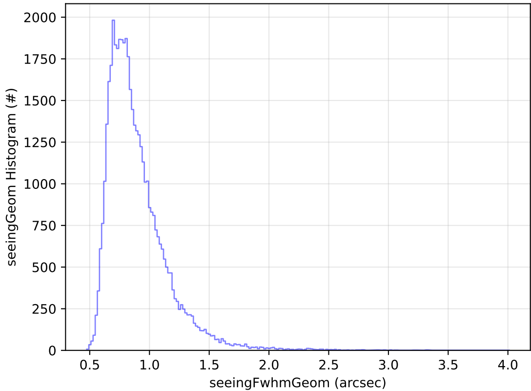
early_ss_template_fpextra2.0_v3.4_10yrs Yr 1 z band: seeingGeom Histogram
