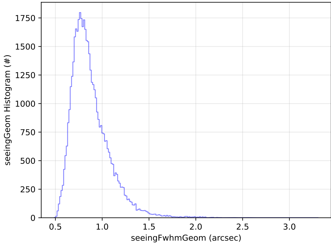
early_ss_template_fpextra2.0_v3.4_10yrs Yr 1 y band: seeingGeom Histogram
