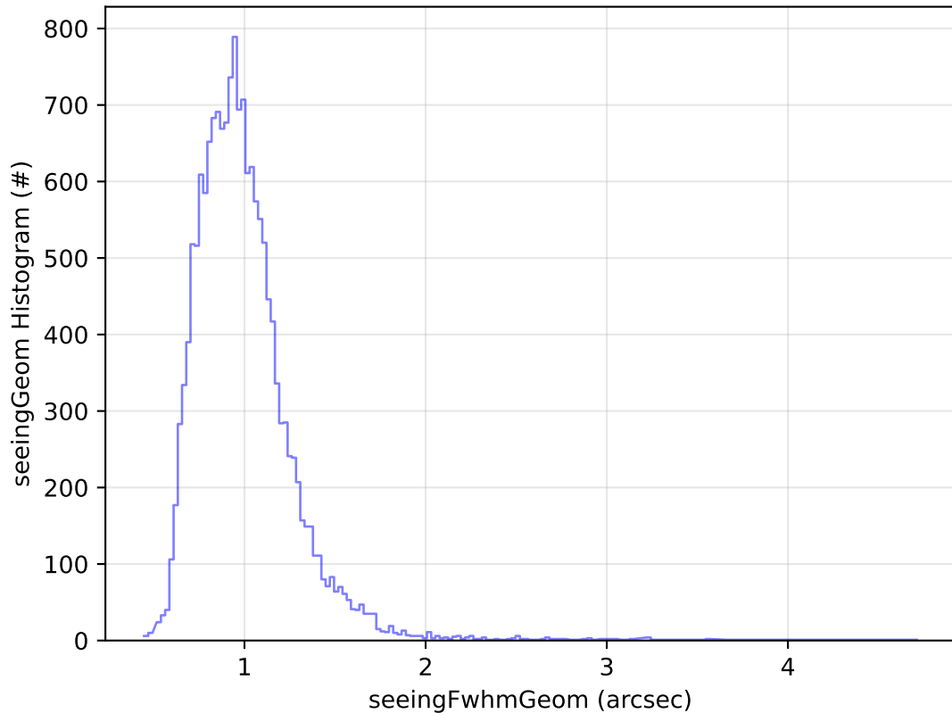
early_ss_template_fpextra2.0_v3.4_10yrs Yr 1 u band: seeingGeom Histogram
