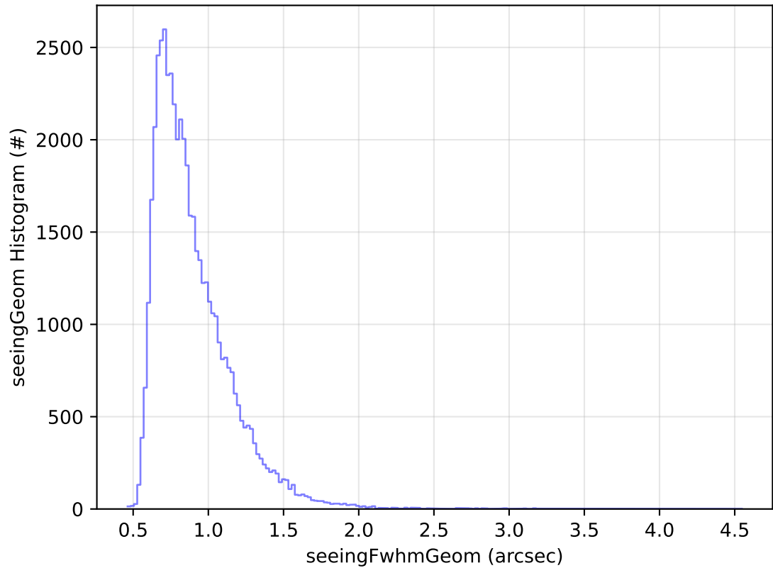
early_ss_template_fpextra2.0_v3.4_10yrs Yr 1 r band: seeingGeom Histogram
