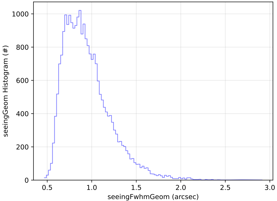
early_ss_template_fpextra2.0_v3.4_10yrs Yr 1 g band: seeingGeom Histogram
