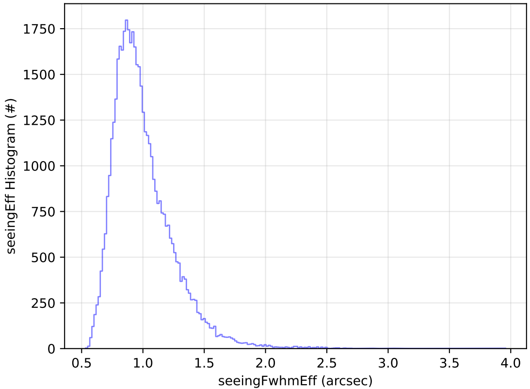
early_ss_template_fpextra2.0_v3.4_10yrs Yr 1 y band: seeingEff Histogram
