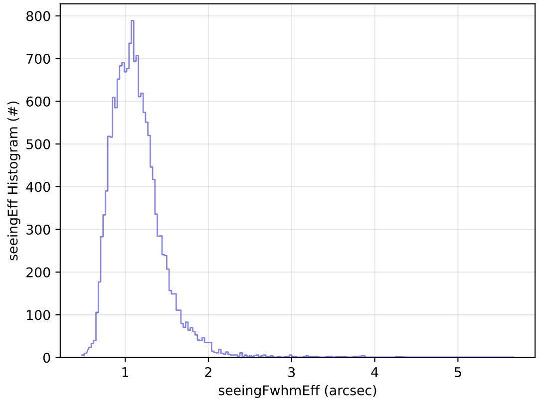
early_ss_template_fpextra2.0_v3.4_10yrs Yr 1 u band: seeingEff Histogram
