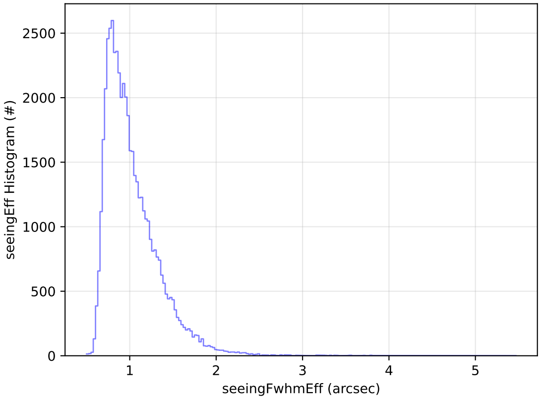
early_ss_template_fpextra2.0_v3.4_10yrs Yr 1 r band: seeingEff Histogram
