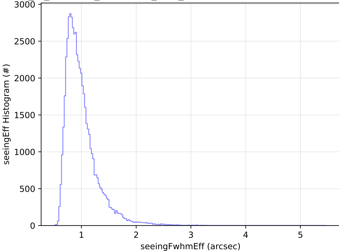
early_ss_template_fpextra2.0_v3.4_10yrs Yr 1 i band: seeingEff Histogram
