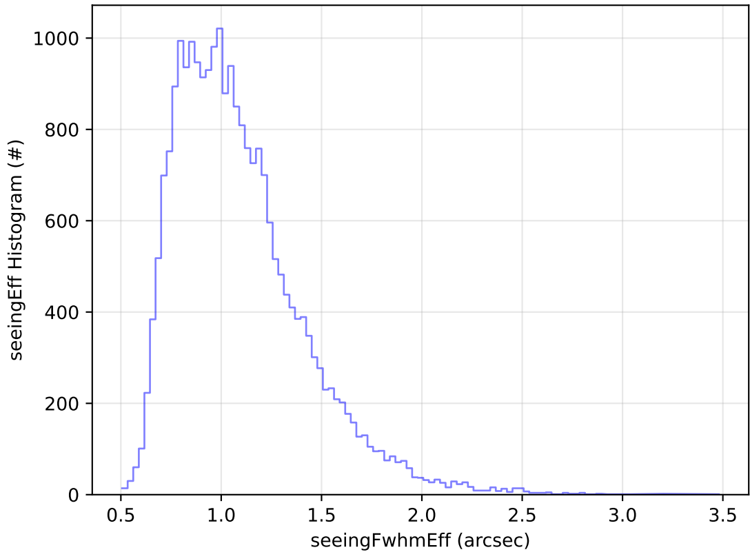
early_ss_template_fpextra2.0_v3.4_10yrs Yr 1 g band: seeingEff Histogram
